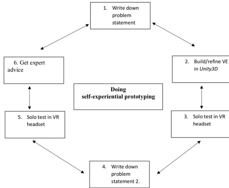
Figure 17: Figure 6. Doing self-experiential prototyping: an iterative cyclic model
